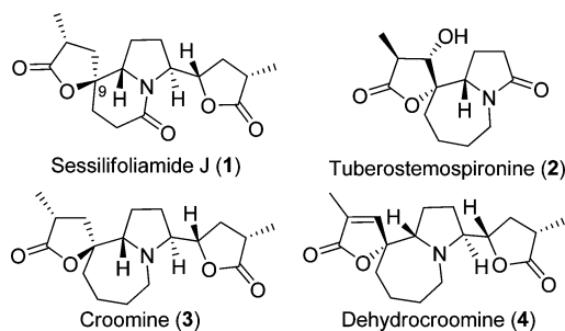
Figure 1. Structures of (–)-sessilifoliamide J ( 1 ) and some tuberostemospironine group alkaloids.
